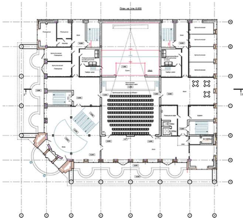
Theatre Moscow suburban area Russian Federation 2009. Team of MARITIMO company; responsibility: design of building and building segments
